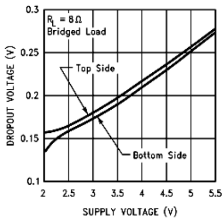
Dropout Voltage vs Supply Voltage
