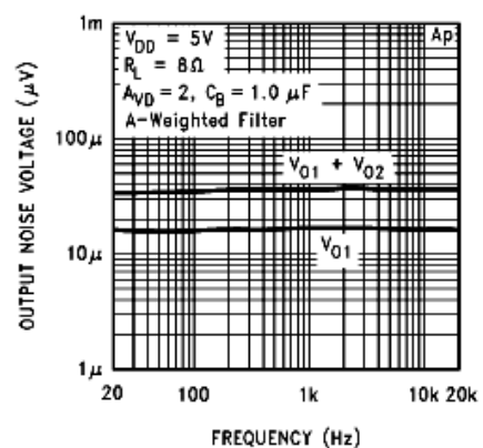
Noise Floor
