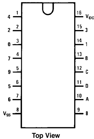
Pin Assignments for DIP and SOP
