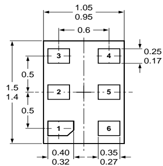
PESDxL5UF (SOT886)
